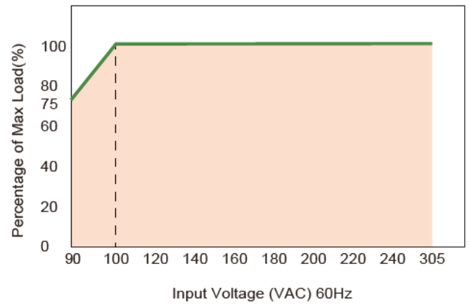
Static Characteristics
